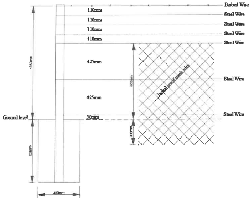
Figure 1 Jackal Proof fence - Wire spacing
