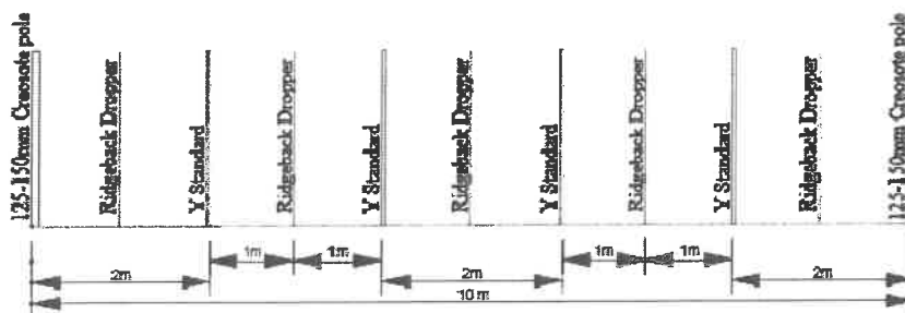
Figure 2 Jackal Proof fence - poles spacing
